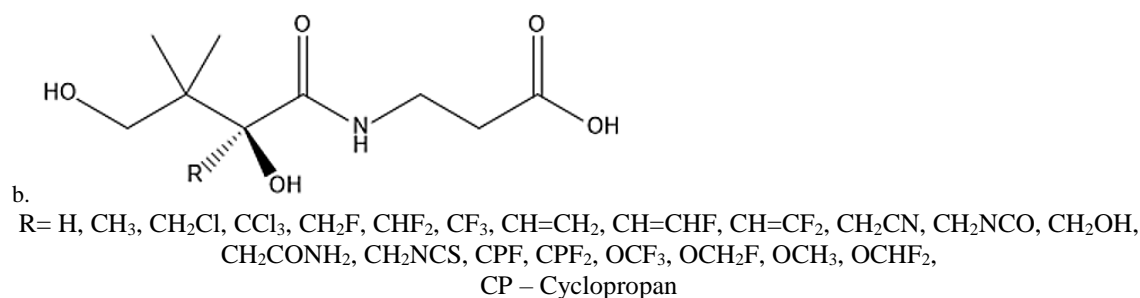
Figure 1. a. i. Molecular structure & ii. Optimized structure of Vitamin B5 (Pantothenic acid), b. Virtually modified derivatives of Vitamin B5
