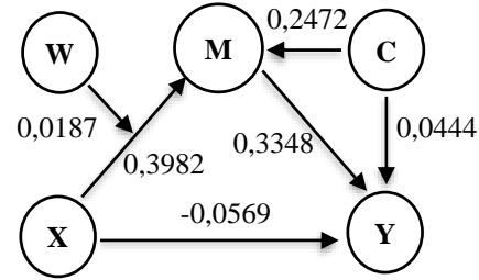
Şekil 10. Moderated mediation analizin covariate değişkenli 7. optimizasyon modelinin kavramsal diyagramı (7. conceptual diagram of the optimization model of moderated mediation analysis with covariate variables)
