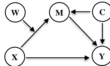
Şekil 9. Moderated mediation analizin covariate değişkenli 7. optimizasyon modelinin kavramsal diyagramı (7. conceptual diagram of the optimization model of moderated mediation analysis with covariate variable)
