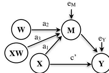
Şekil 8. Moderated mediation analizin 7. Optimizasyon modelinin istatistiksel diyagramı (7. statistical diagram of the optimization model of moderated mediation analysis)
