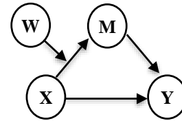
Şekil 7. Moderated mediation analizin 7. Optimizasyon modelinin kavramsal diyagramı (7. conceptual diagram of the optimization model of moderated mediation analysis)
