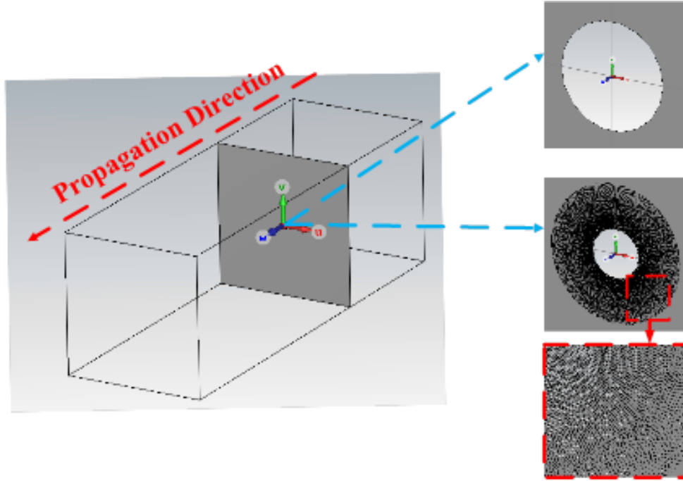
Figure 6. An overview of the CST model of the AMDL and MDL (AMDL ve MDL'nin CST modeline genel bakış)
