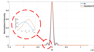
a) Comparison of intensity distributions
