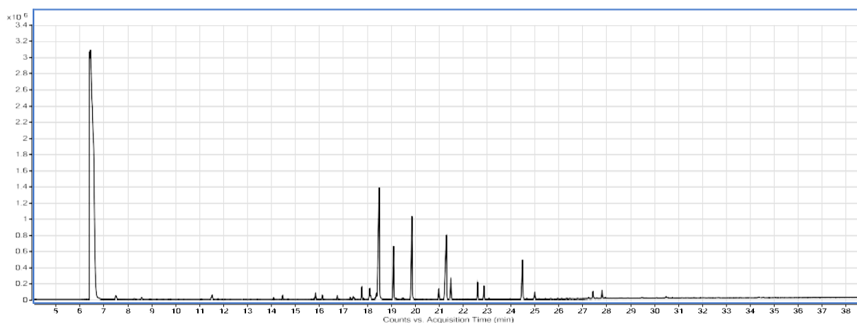
Figure 6. Gas Chromatography of Rosa damascena L. Essential Oil
