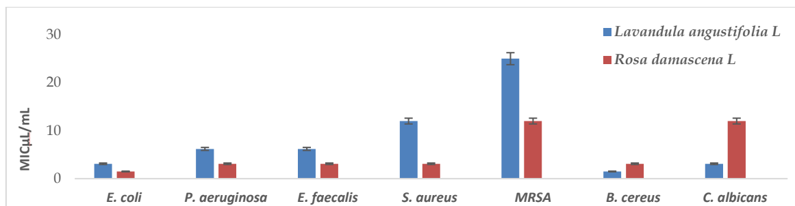
Figure 5. MIC Values of lavender and rose oils
