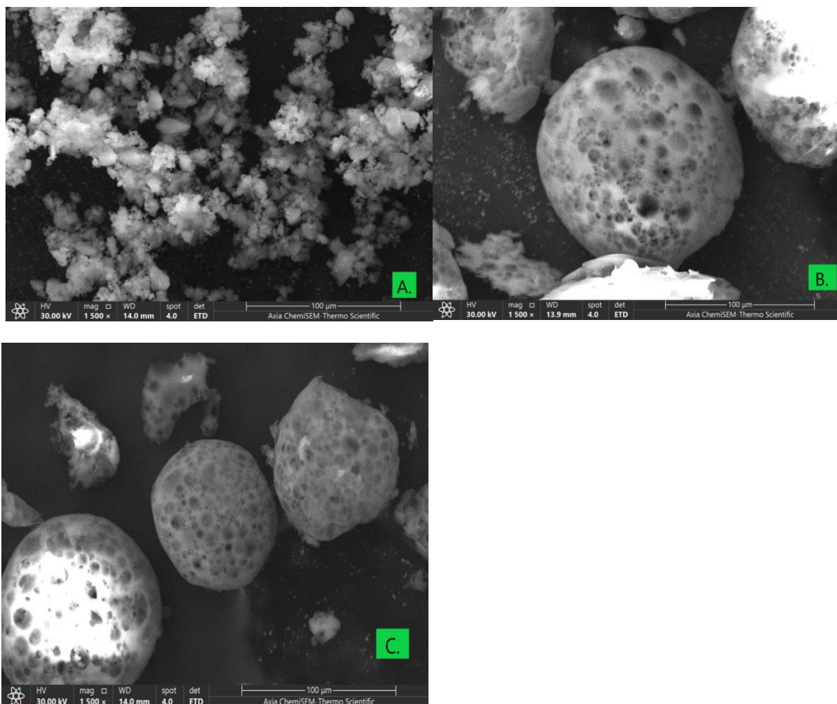
Figure 1. SEM pictures at 1500 mag of A) CP. B) F1 and C) F2.
