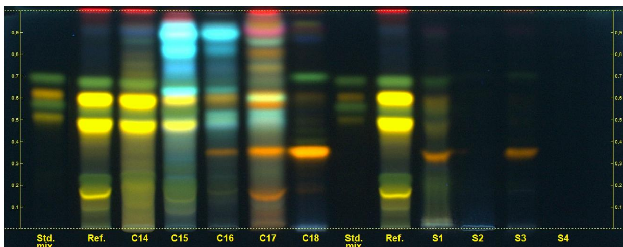
Figure 3. HPTLC chromatogram of hydroalcoholic extract of the reference plant material (Ref.) and P. incarnata extract containing products including capsule/tablet/powder (C14-18) and syrups (S1-4) sold in the market captured at 366 nm after derivatization with NP and PEG reagents, respectively.
