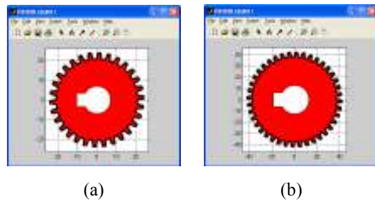
Figure 6. Pinion gear samples, a) Module=1.5, teeth number=30, b) Module=2, teeth number=40.
