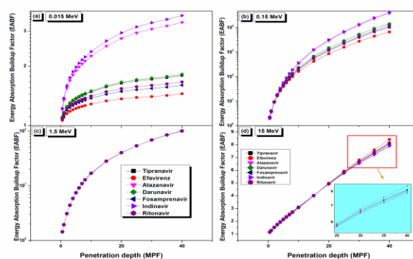
Figure 7. The EABF values for the investigated drugs up to 40 MFP at 0.015, 0.15, 1.5, and 15 MeV.
