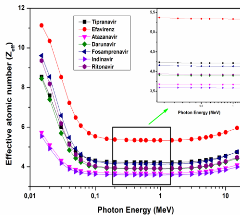
Figure 4. The variations in the investigated drugs' Z_{\text{eff}} values versus the incoming photon energy.
