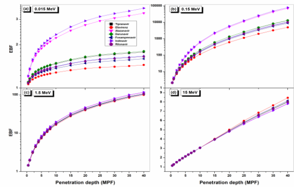
Figure 6. The EBF values for the investigated drugs up to 40 MFP at 0.015, 0.15, 1.5, and 15 MeV.
