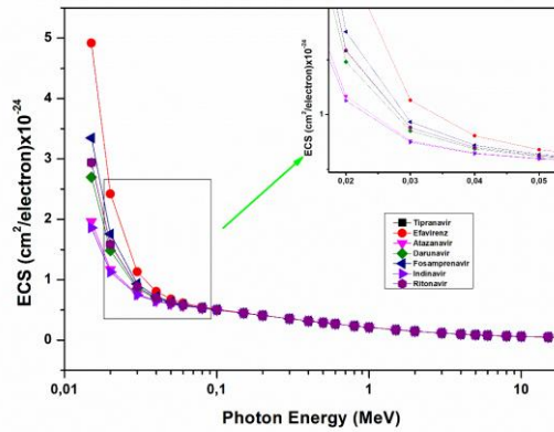
Figure 3. The variations in the investigated drugs' ECS values versus the incoming photon energy.
