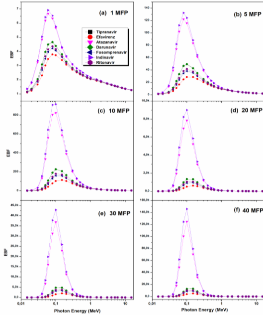
Figure 5. The variations in EBF with photon energy at 1, 5, 10, 20, 30, and 40 MFP for the investigated drugs.
