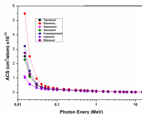
Figure 2. The changes in ACS values of drugs according to incoming photon energy.
