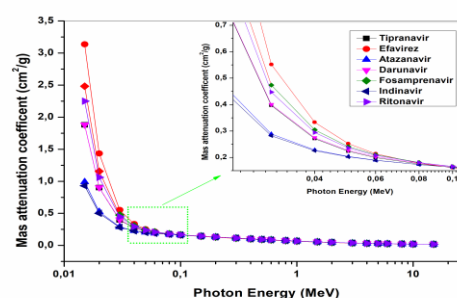
Figure 1. The investigated drugs' MAC values differ from the incoming photon energy.
