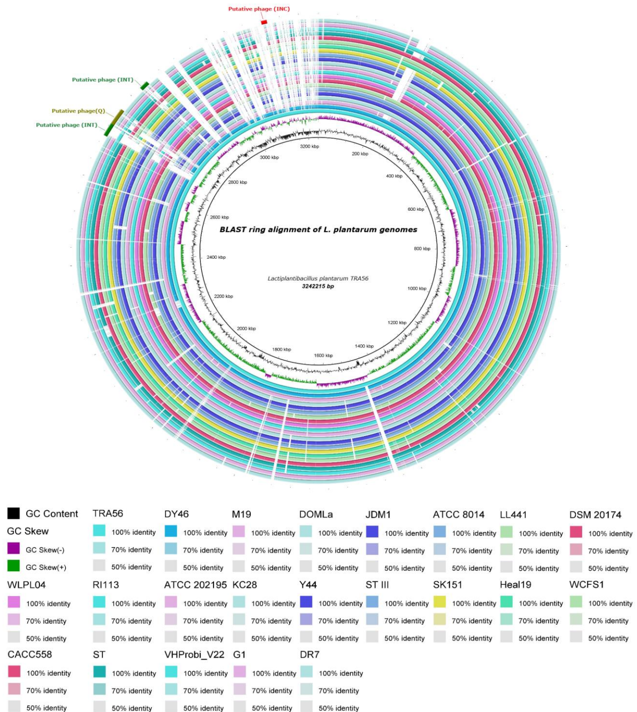
Figure 1. BLAST ring alignment of Lactiplantibacillus plantarum genomes. The genomes are sorted from in inner turquoise ring(TRA56) to the outer sky blue ring(DR7). The GC skew (+/-) of the TRA56 genome was displayed in the third inner circle, while the GC content was illustrated in the second inner circle. The genome size was also shown in the first inner circle, preceding the GC content. Prophage regions in the TRA56 genome are represented as different colored arcs [Intacts (INC): green, Questionable (Q): olive, Incomplete (INC): red].
