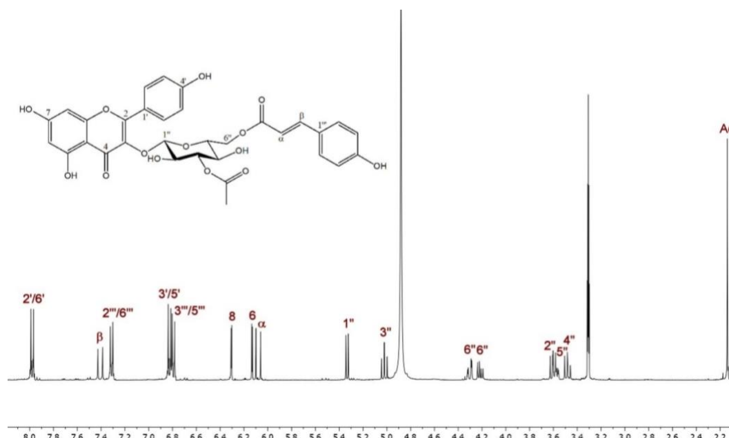
Figure 2. ^1\text{H} NMR Spectrum (400 MHz, \text{CD}_3\text{OD} ) of 8 .
