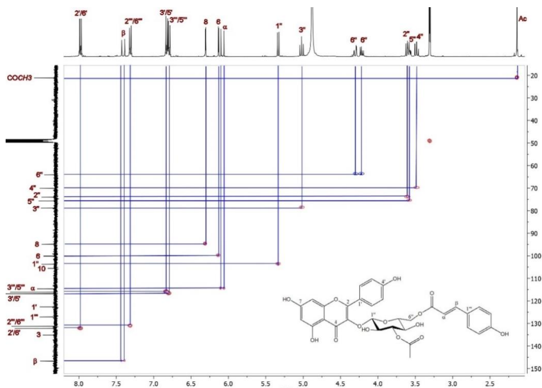
Figure 4. HSQC Spectrum of 8.
