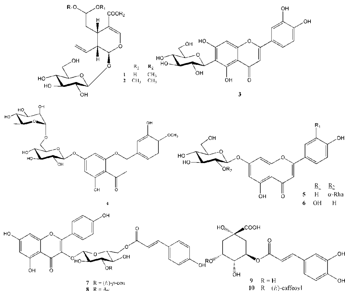
Figure 1. Chemical structures of compounds 1-10 isolated from S. atropurpurea .
