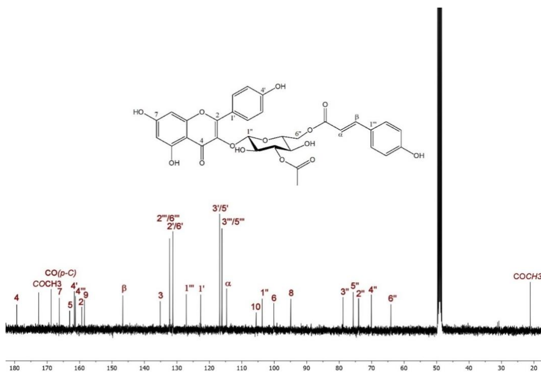
Figure 3. ^{13}\text{C} NMR Spectrum (100 MHz, \text{CD}_3\text{OD} ) of 8 .
