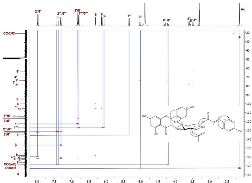
Figure 5. HMBC Spectrum of 8.
