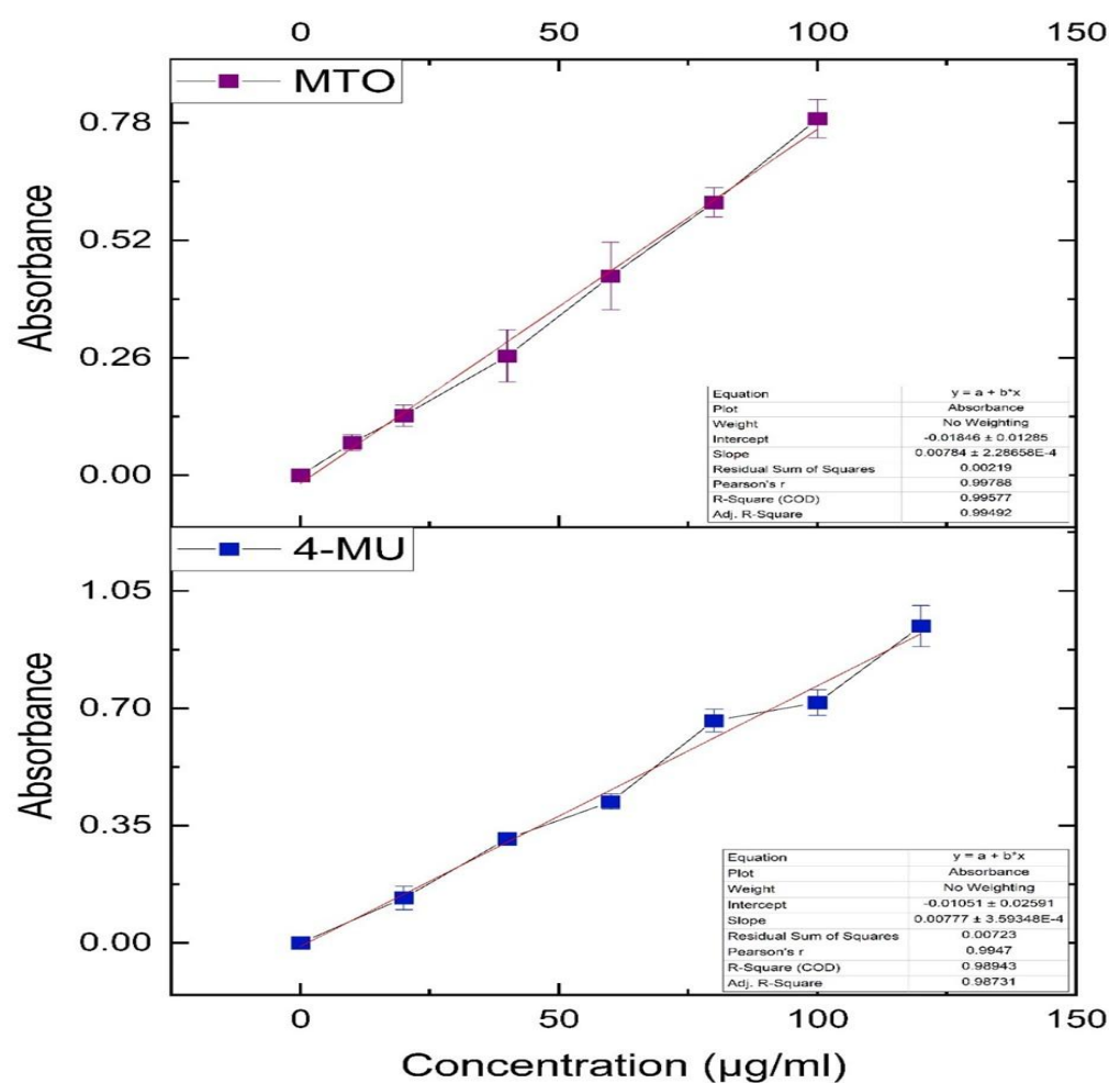
Figure 1. Calibration Plot for MTO in double distilled water at 269 nm and 4-MU in methanol and water(1:1) at 320 nm.
